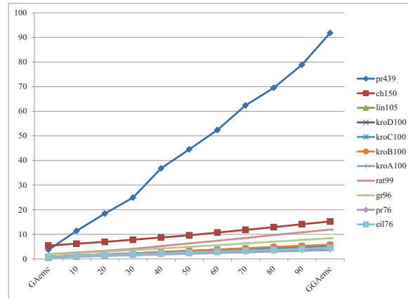
Figure 3.2: The running time as a function of amount of hybridization.
