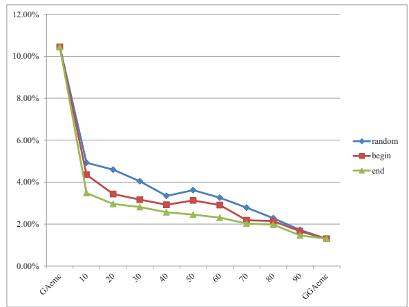
Figure 3.3: Quality results for case pr439 as the amount of hybridization increases.
