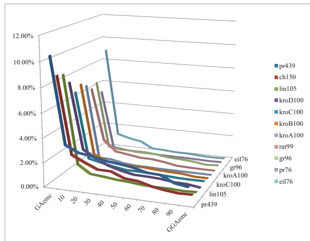
Figure 3.4: Quality results for all cases using end-hybridization.
