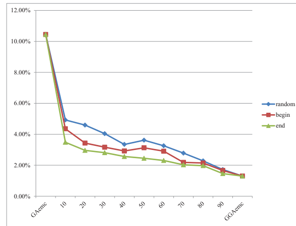
Figure 3.3: Quality results for case pr439 as the amount of hybridization increases.
