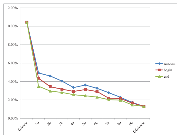
Figure 3.5: Quality results for case pr439 as the amount of hybridization increases.
